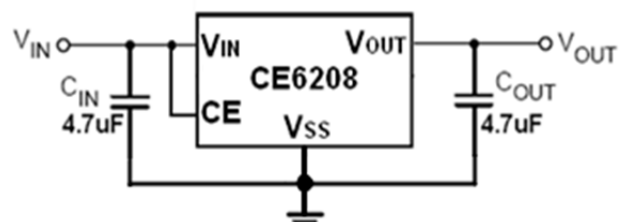
Figure2 CE6208B Typical Application Circuit
