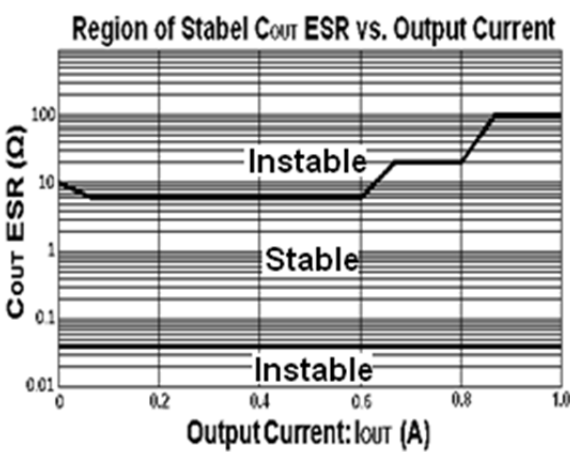
(4) Region of Stable C_{OUT} ESR vs. Load
