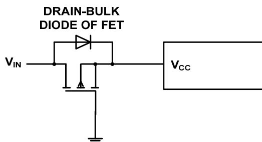
Figure 14. Low Loss Input Reverse Polarity Protection
