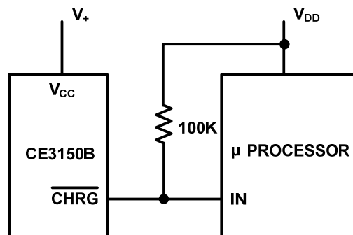
Figure 13. Using a Microprocessor to Determine \overline{\text{CHRG}} State
