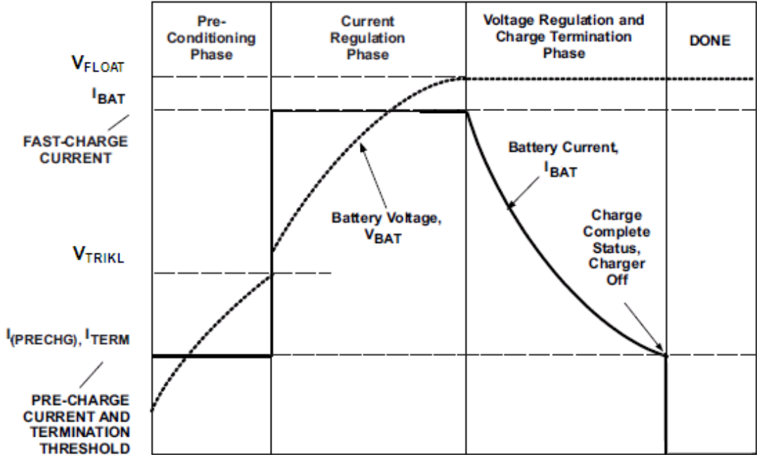
Figure 3. Charging Profile With T_{\text{J(REG)}}
