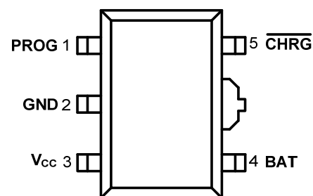
SOT89-5 (Top View)
