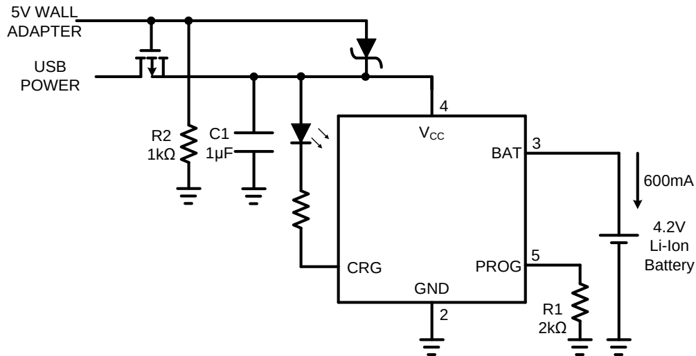
Figure1 Basic Application Circuit
