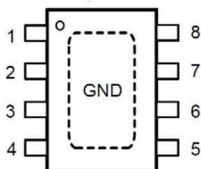
SOP8-PP(Top View)
