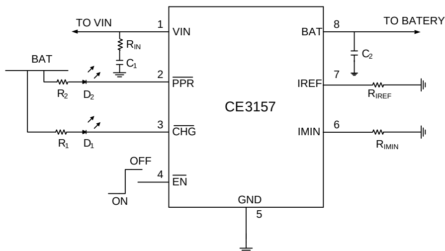
Figure1 Typical Application Circuit Interfacing to Indication LEDs
