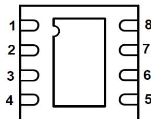
DFN3X3-8(Top View)
