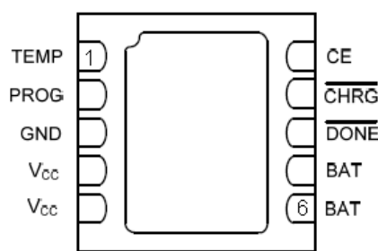
DFN3X3-10(Top View)
