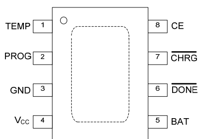
SOP8-PP(Top View)
