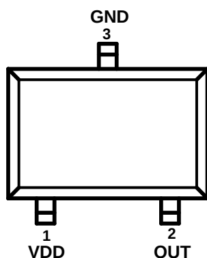
SOT23-3 (Top View)
