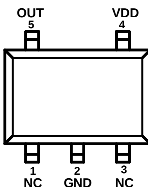
SOT23-5 (Top View)
