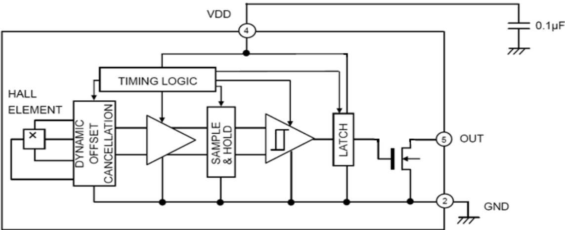
Figure 3. CE100XN Functional Block Diagram
