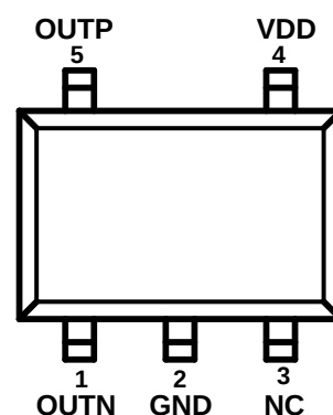
SOT23-5 (Top View)
