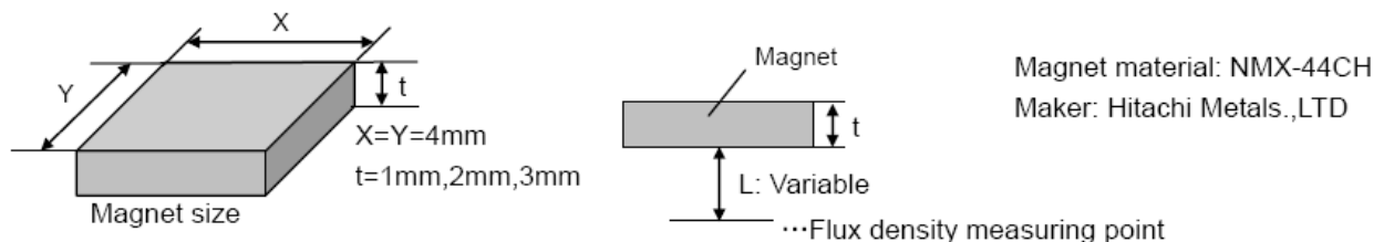
Figure 8. Magnet Hall IC Distance
