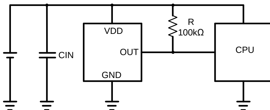
Figure 1. Standard Application Circuit (CE100XN)
