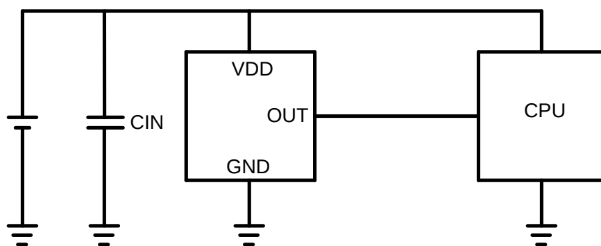
Figure 2. Standard Application Circuit (CE100XC)
