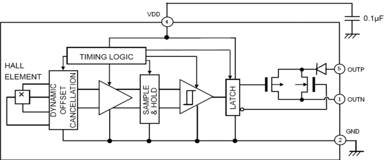
Figure 5. CE1014 Functional Block Diagram
