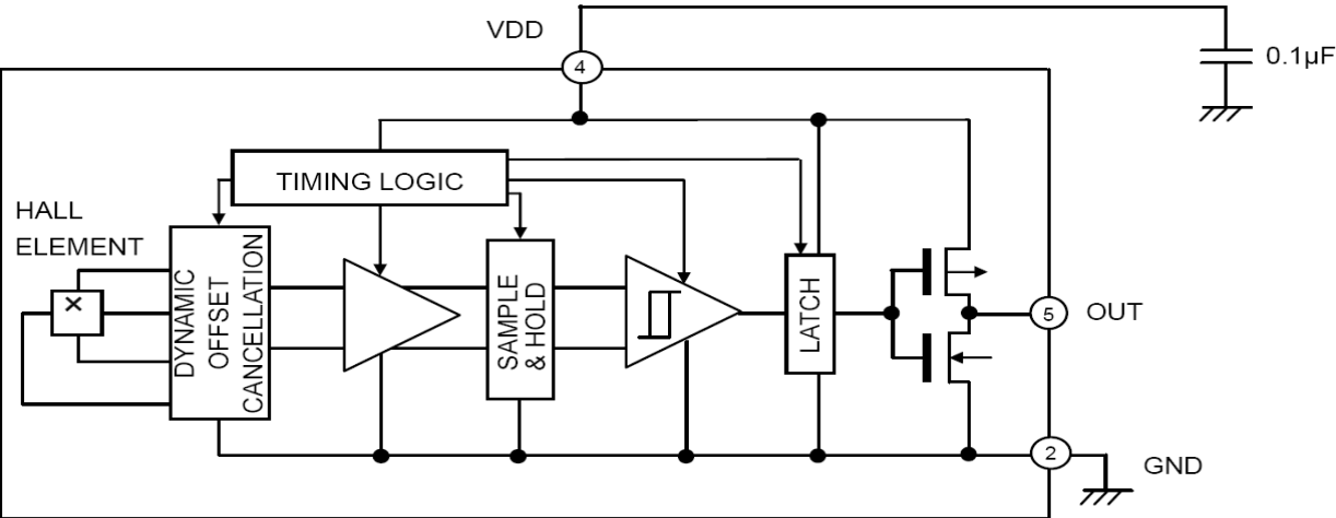
Figure 4. CE100XC Functional Block Diagram
