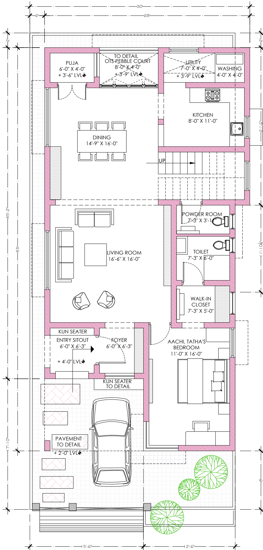
SCHEMATIC - GROUND FLOOR PLAN SIVA SAKTHI Residence - Sivakasi
