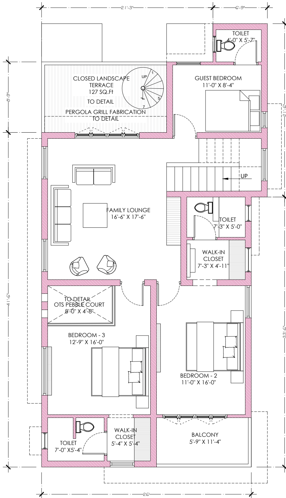
SCHEMATIC - FIRST FLOOR PLAN SIVA SAKTHI Residence - Sivakasi
