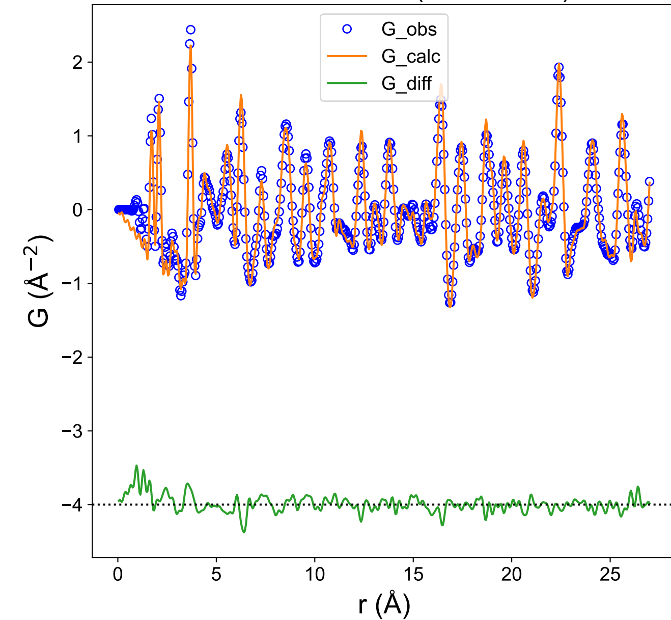
PDF Data and Fit (Rw = 0.190)
