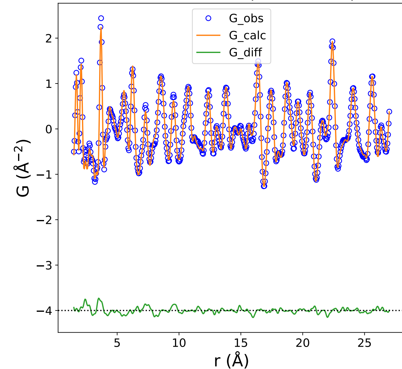
PDF Data and Fit (Rw = 0.108)
