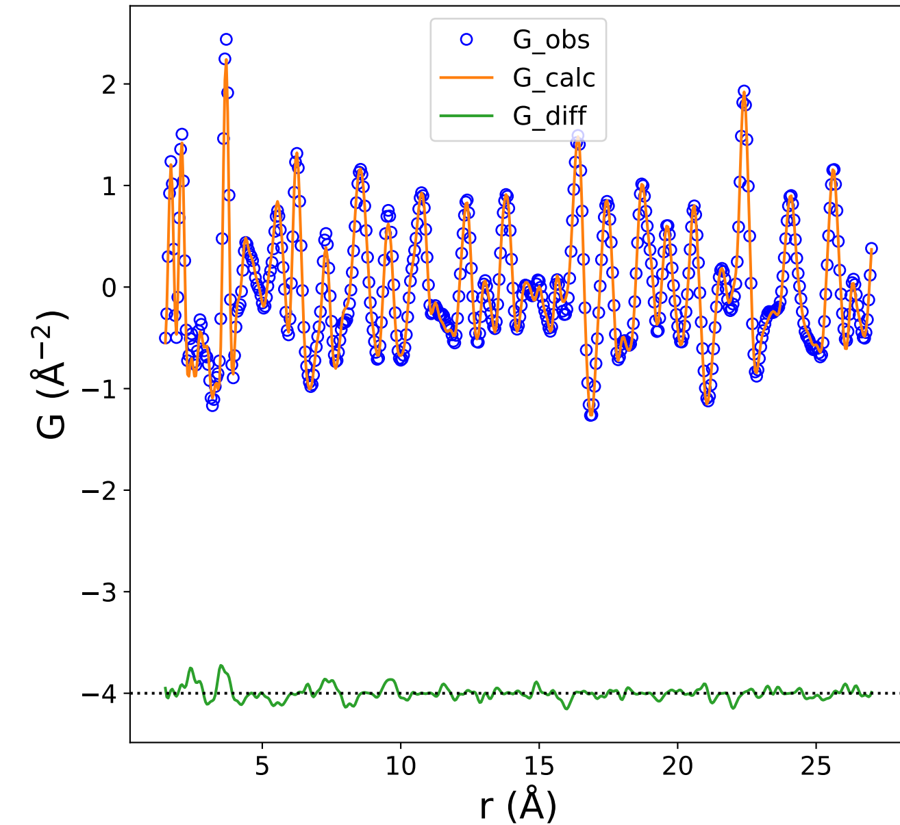
PDF Data and Fit (Rw = 0.107)
