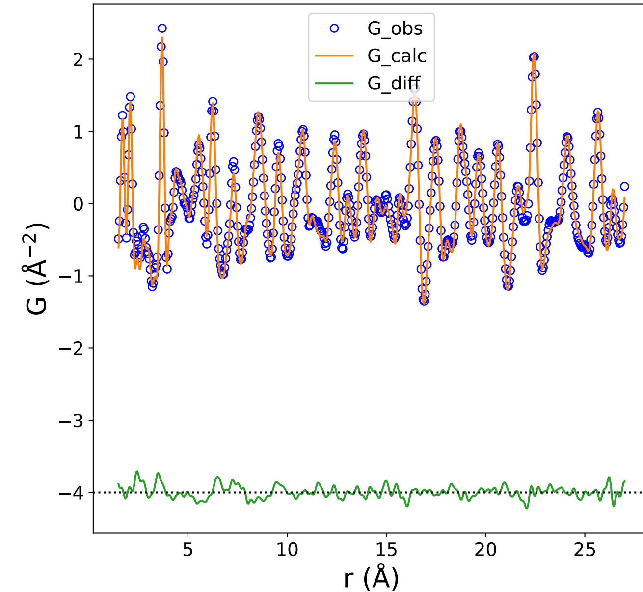
PDF Data and Fit (Rw = 0.135)
