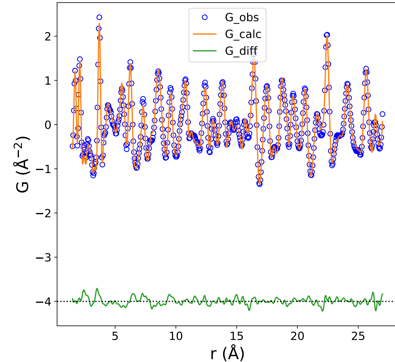
PDF Data and Fit (Rw = 0.131)
