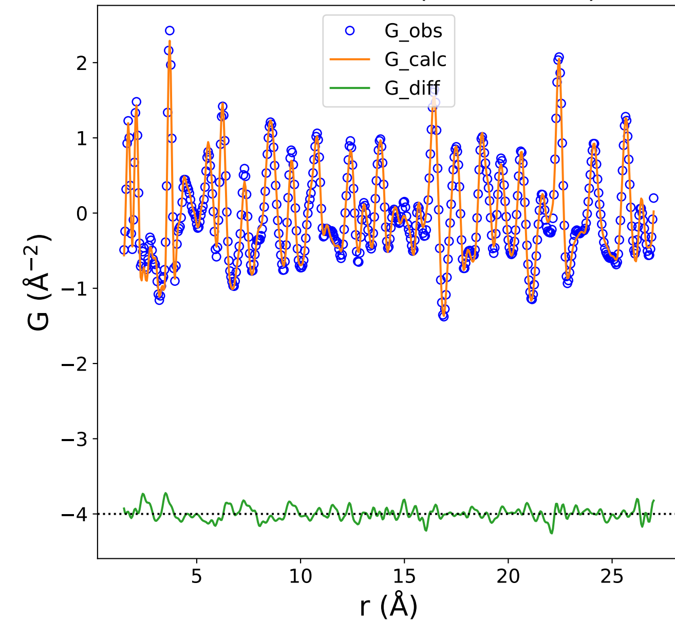
PDF Data and Fit (Rw = 0.133)
