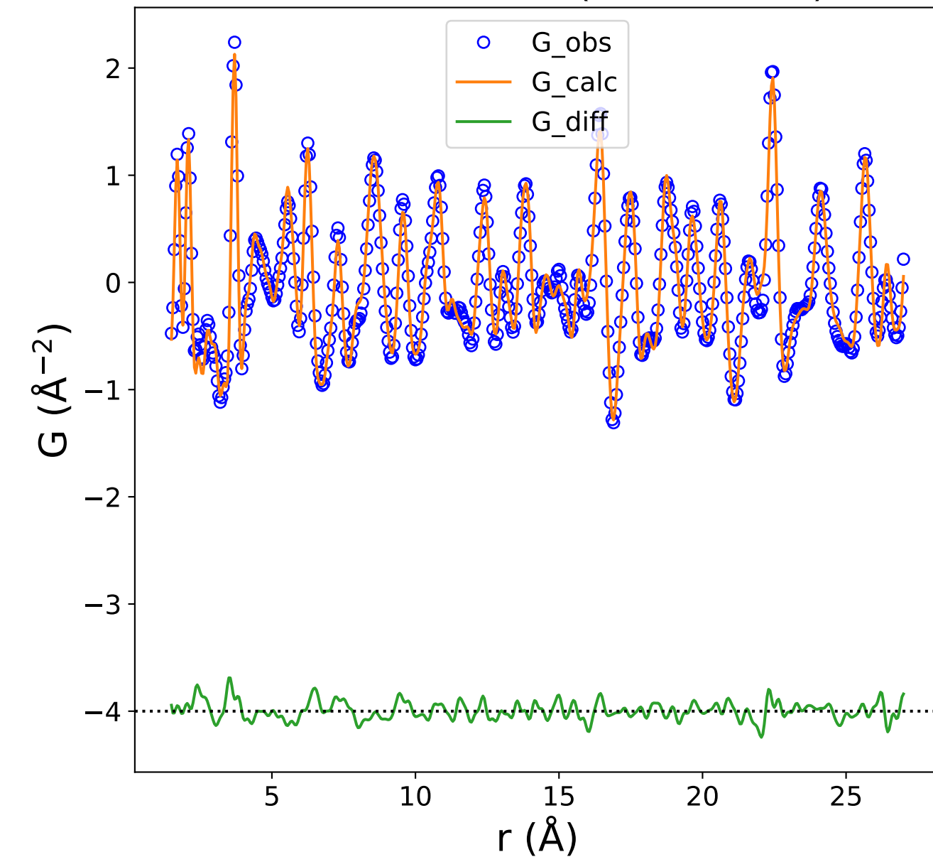
PDF Data and Fit (Rw = 0.138)
