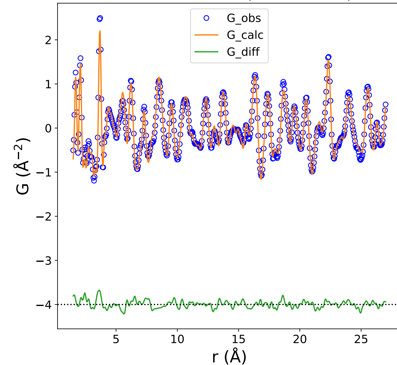
PDF Data and Fit (Rw = 0.152)
