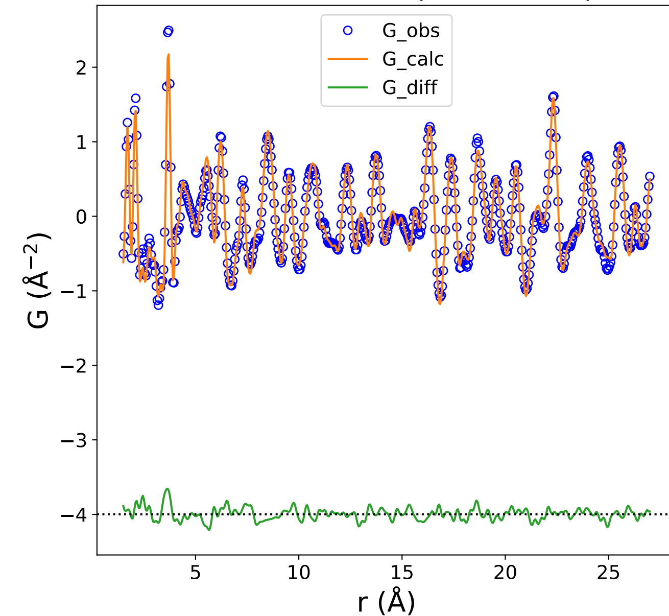
PDF Data and Fit (Rw = 0.147)
