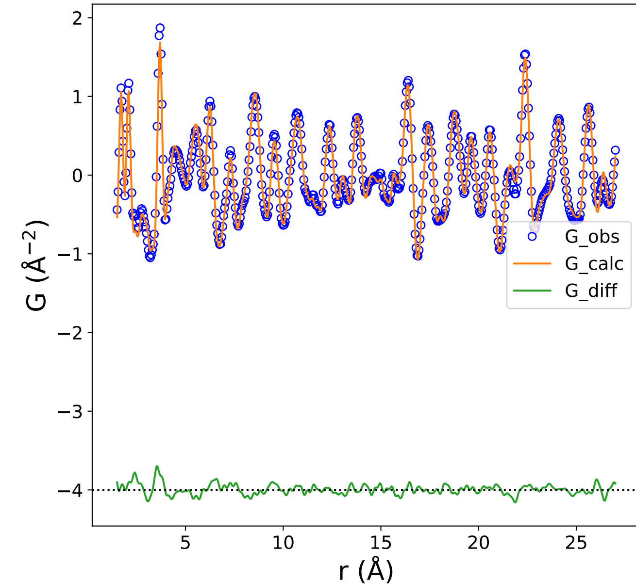
PDF Data and Fit (Rw = 0.130)
