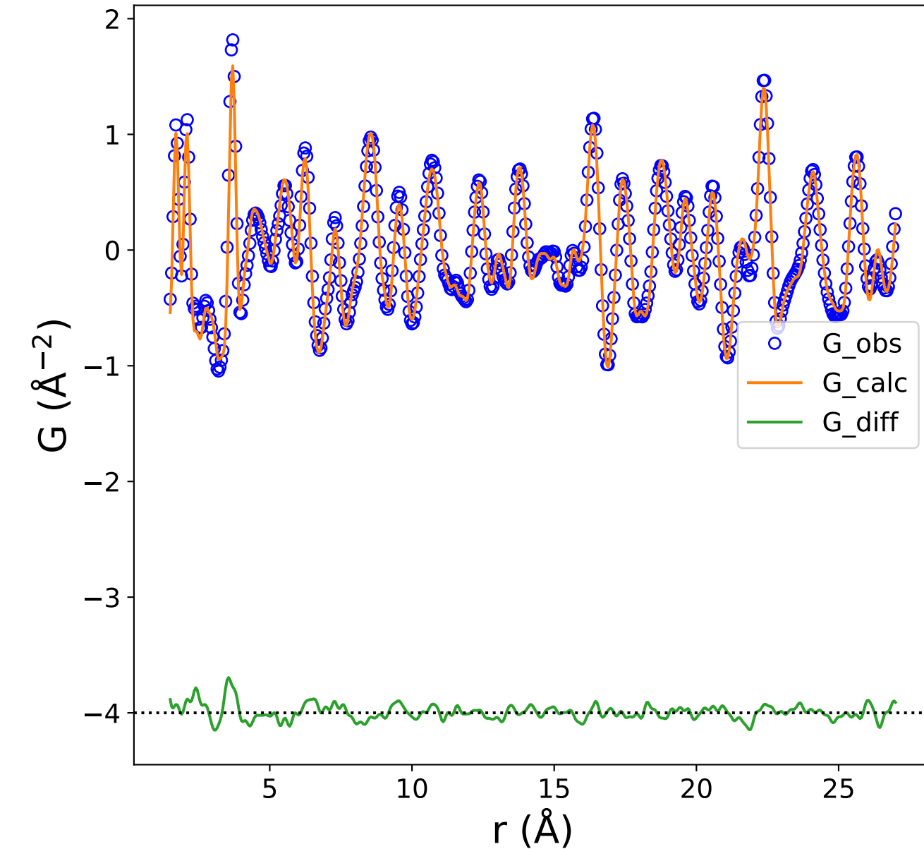
PDF Data and Fit (Rw = 0.132)
