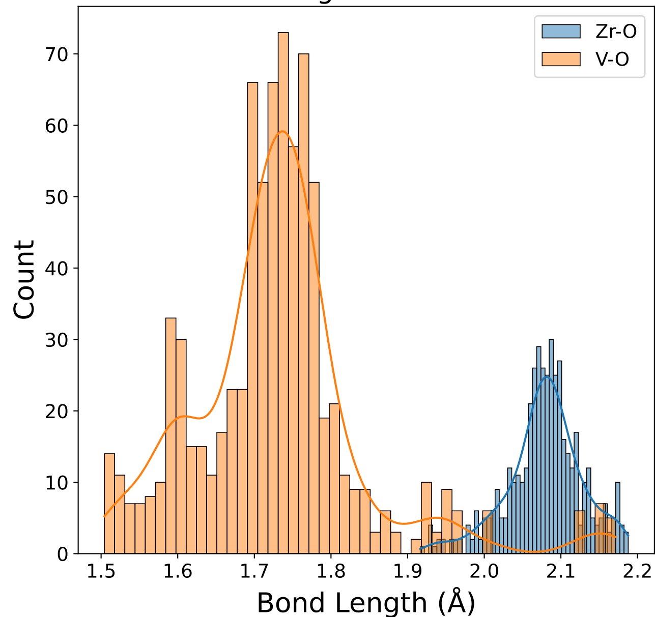
Bond Length Distributions
