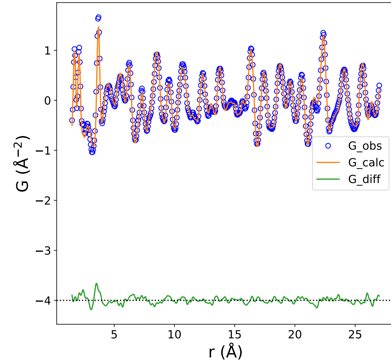
PDF Data and Fit (Rw = 0.149)
