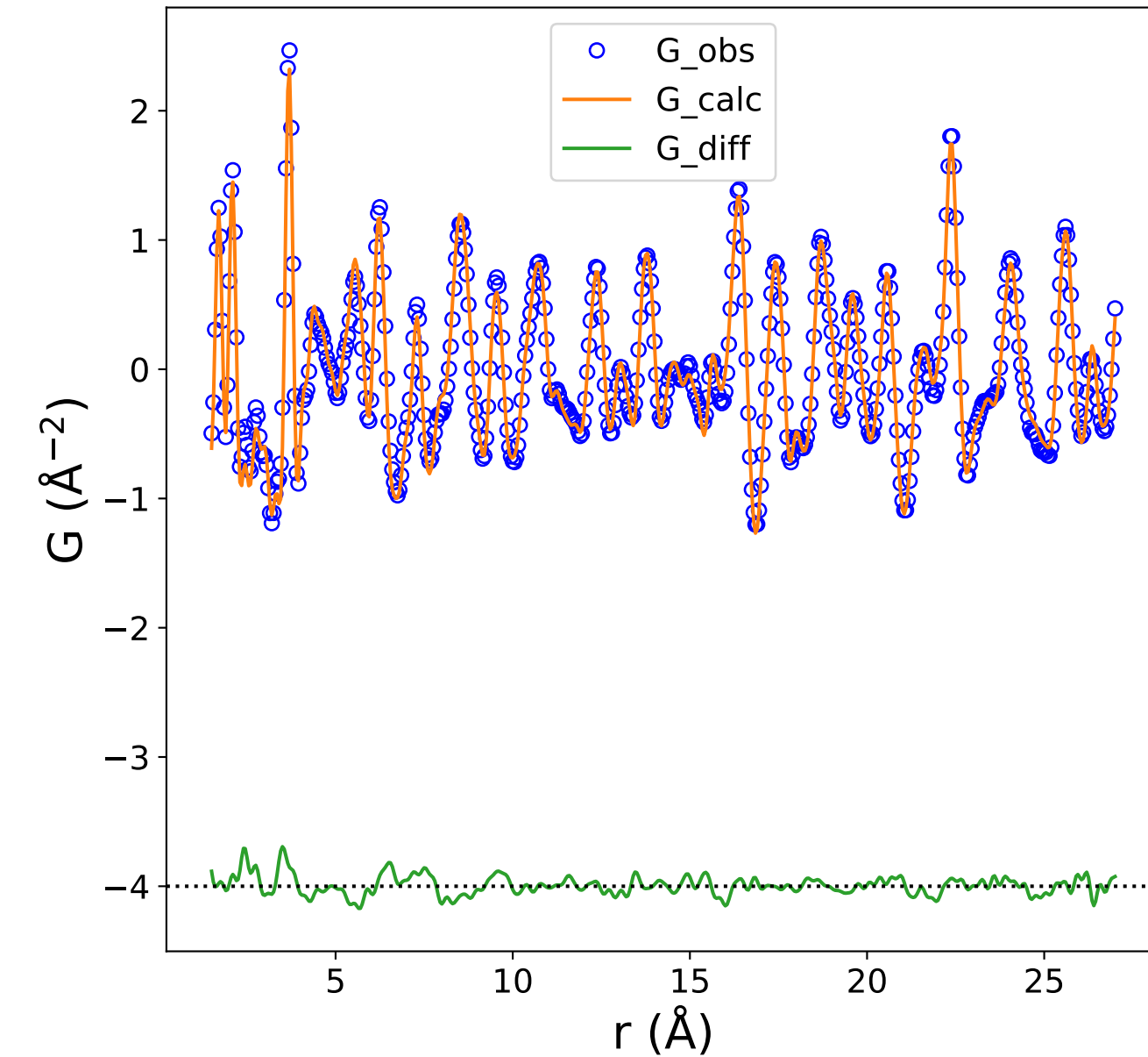
PDF Data and Fit (Rw = 0.124)
