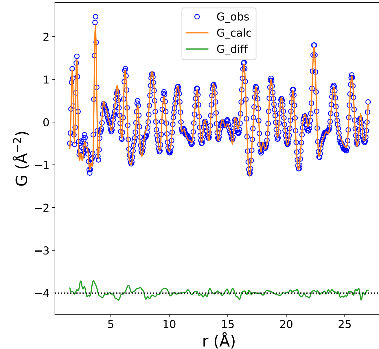
PDF Data and Fit (Rw = 0.123)
