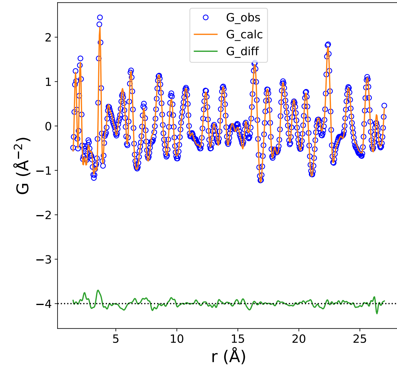
PDF Data and Fit (Rw = 0.117)
