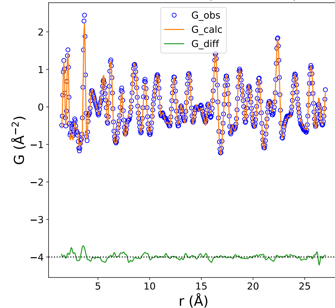
PDF Data and Fit (Rw = 0.114)
