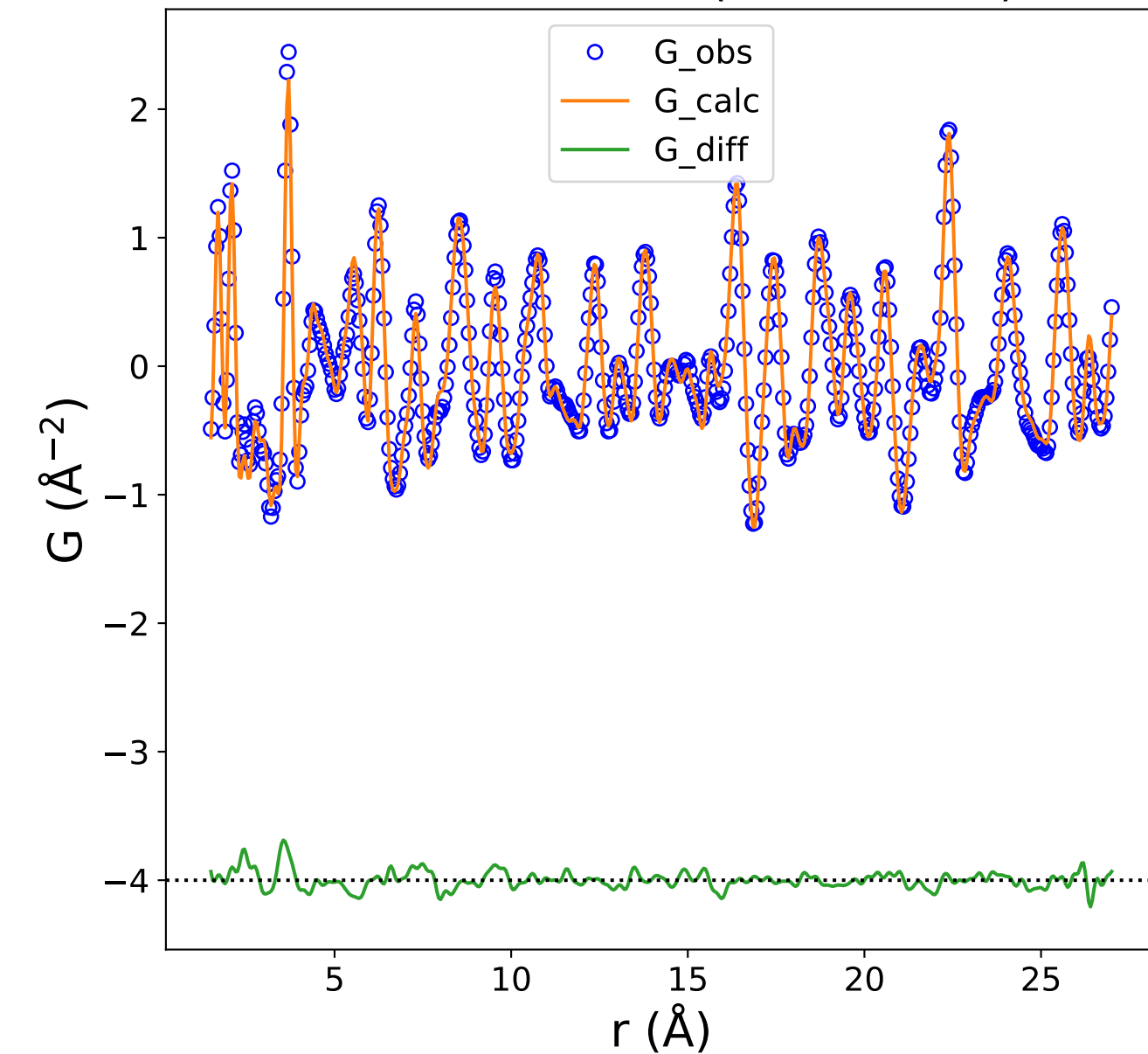
PDF Data and Fit (Rw = 0.113)
