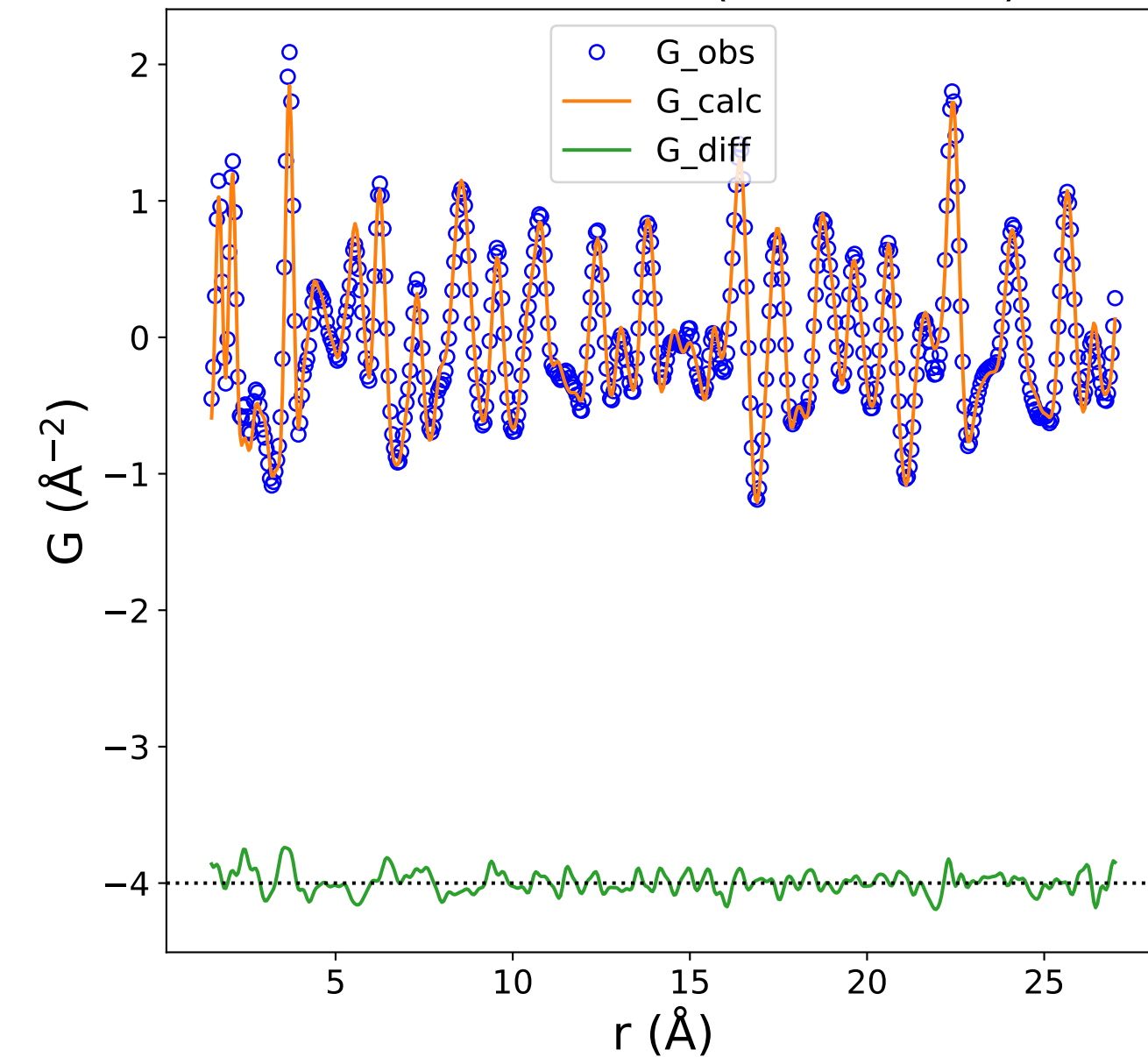
PDF Data and Fit (Rw = 0.142)
