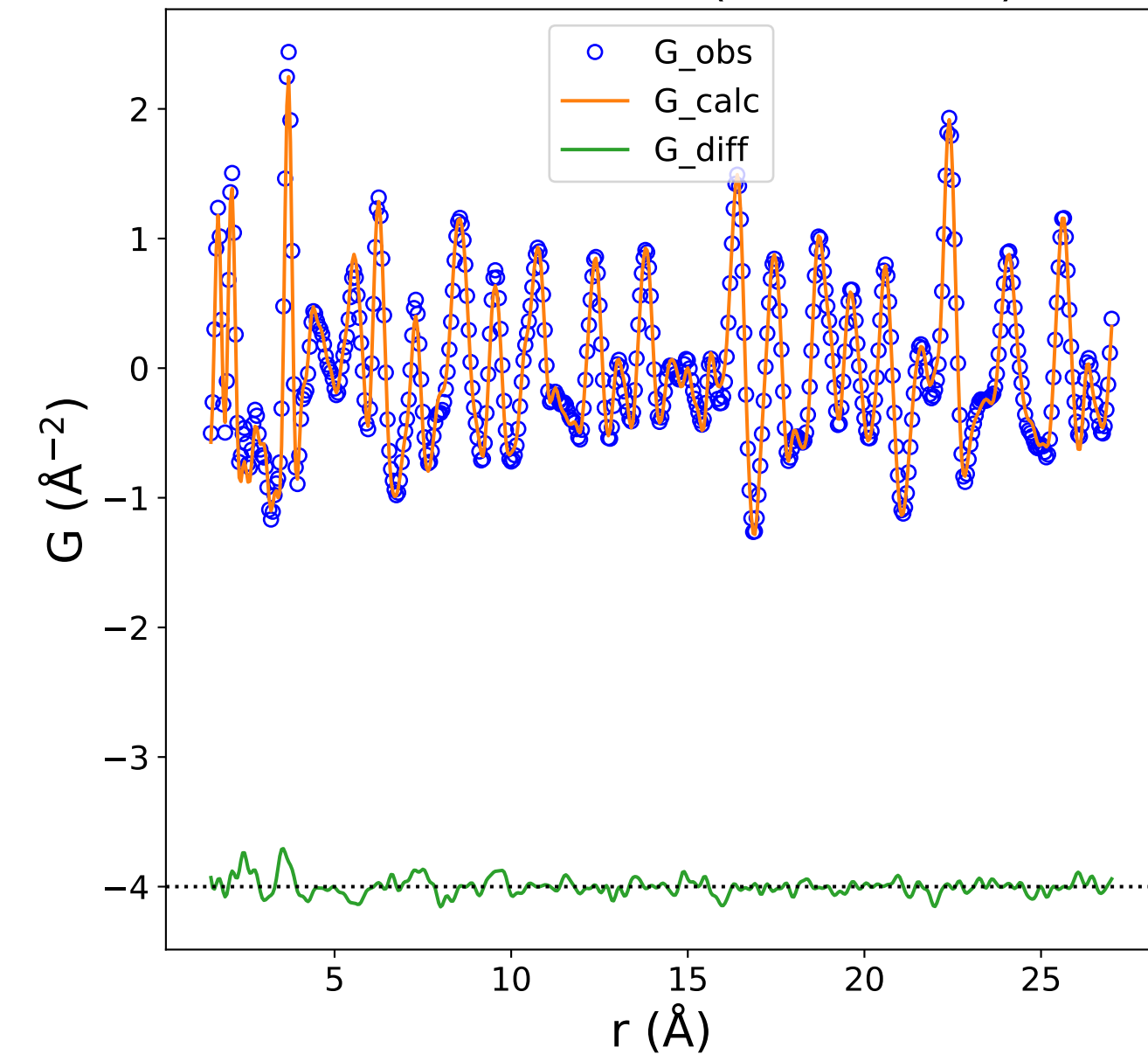
PDF Data and Fit (Rw = 0.111)
