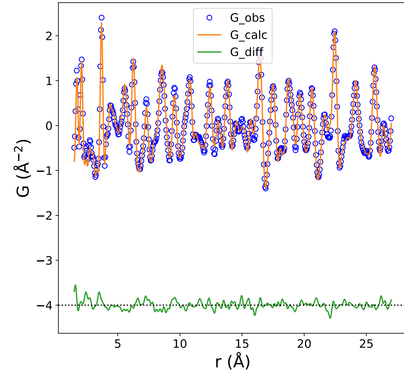
PDF Data and Fit (Rw = 0.151)
