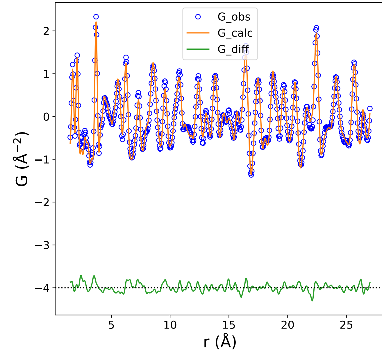
PDF Data and Fit (Rw = 0.150)
