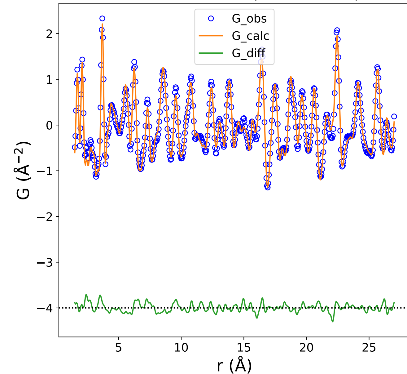
PDF Data and Fit (Rw = 0.148)
