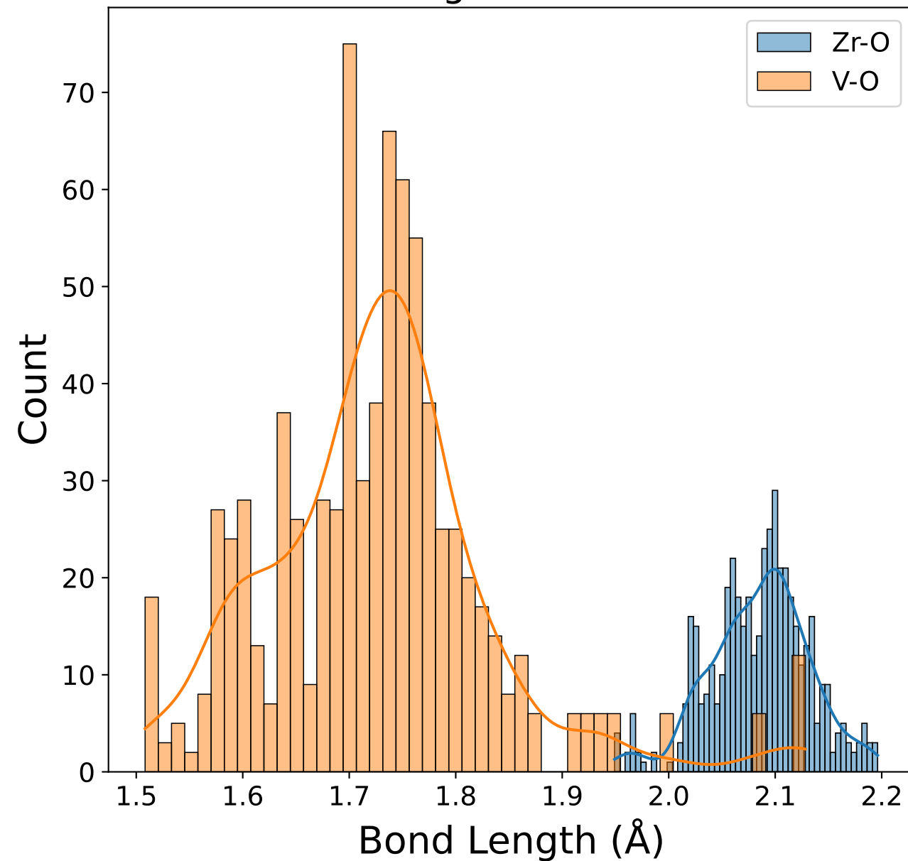
Bond Length Distributions
