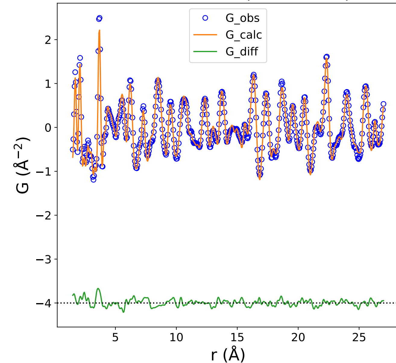
PDF Data and Fit (Rw = 0.143)
