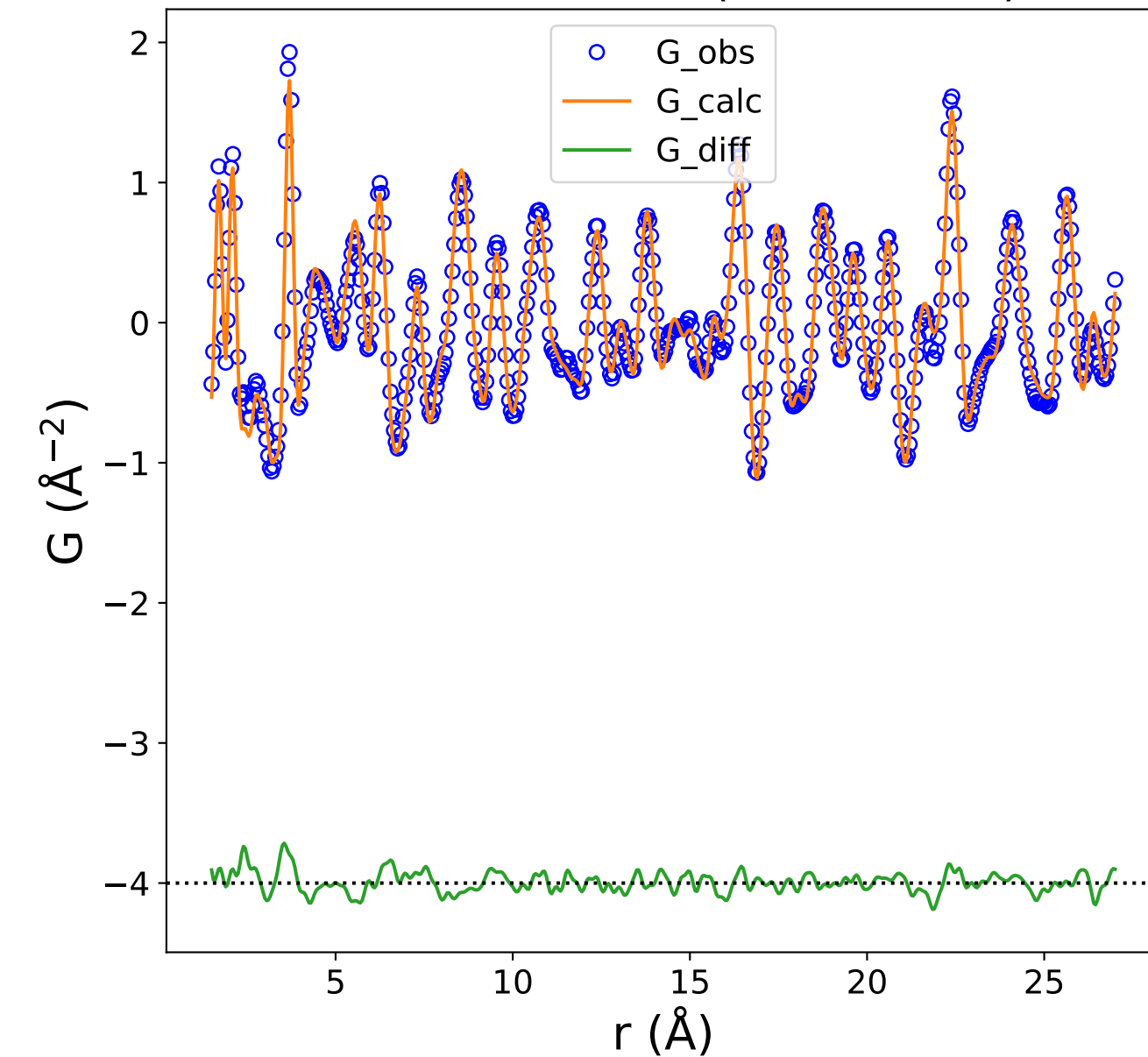
PDF Data and Fit (Rw = 0.140)
