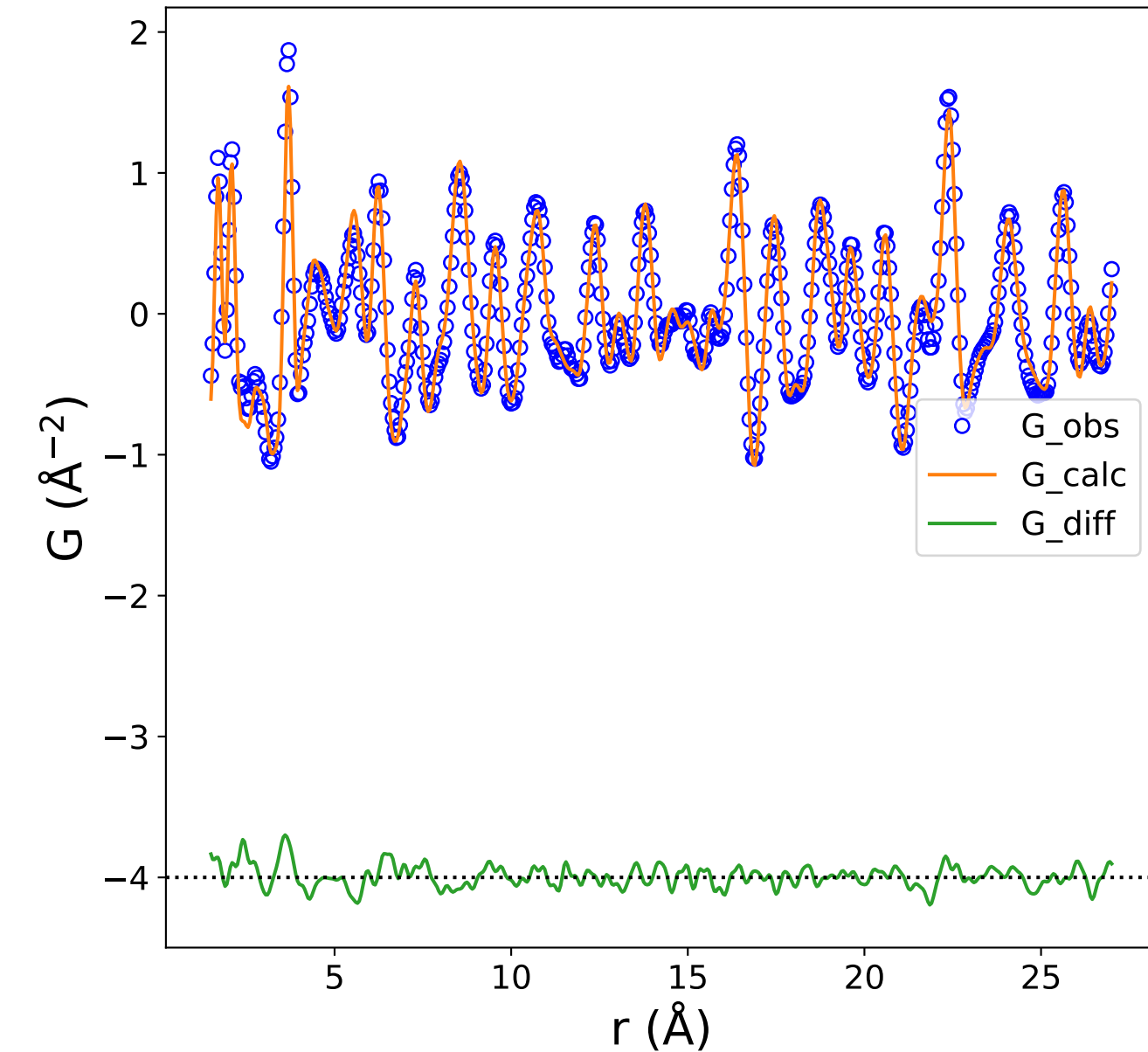
PDF Data and Fit (Rw = 0.154)
