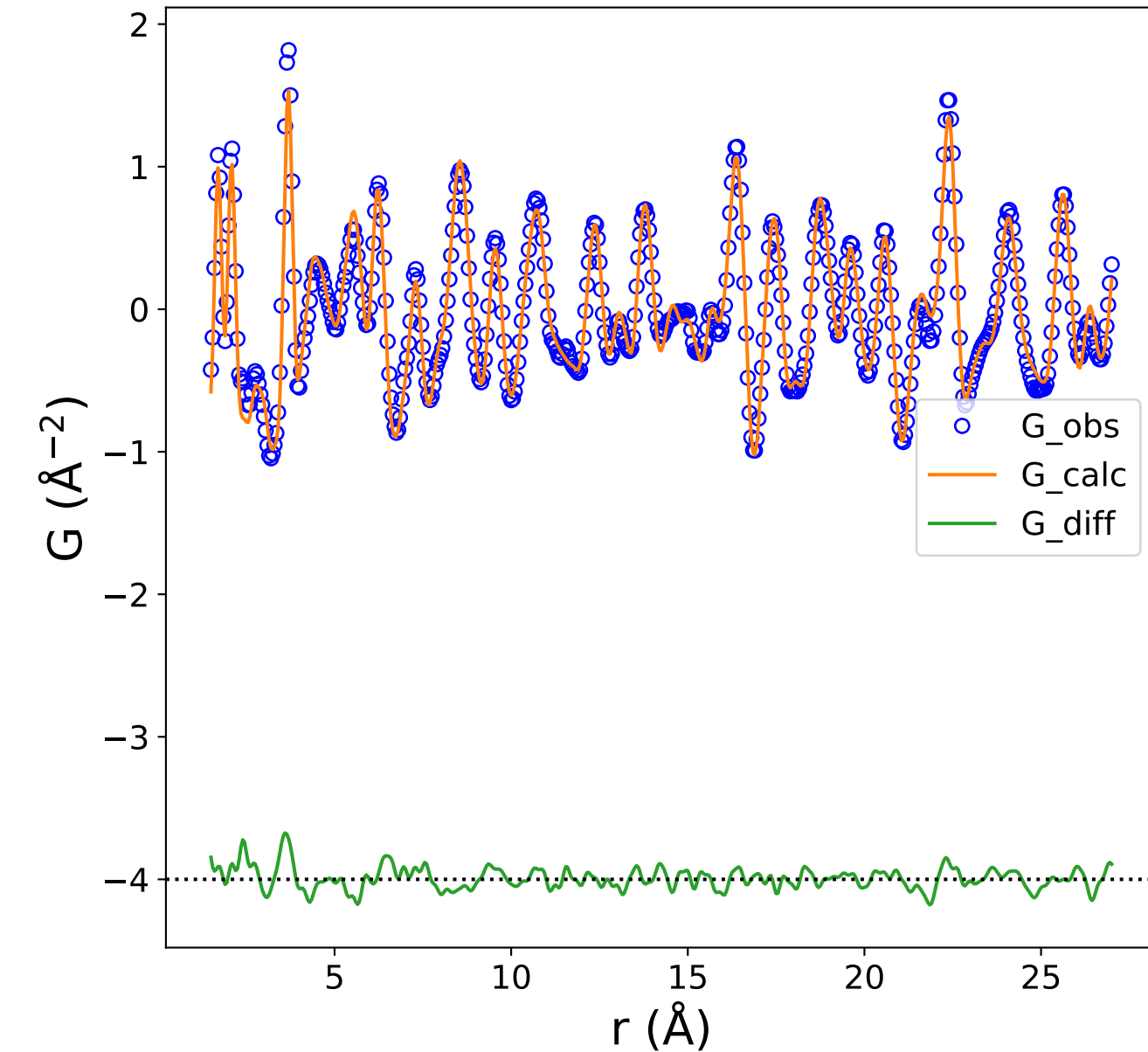
PDF Data and Fit (Rw = 0.155)
