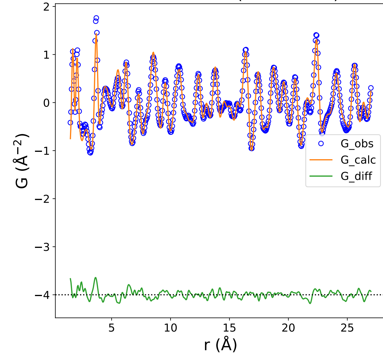
PDF Data and Fit (Rw = 0.174)
