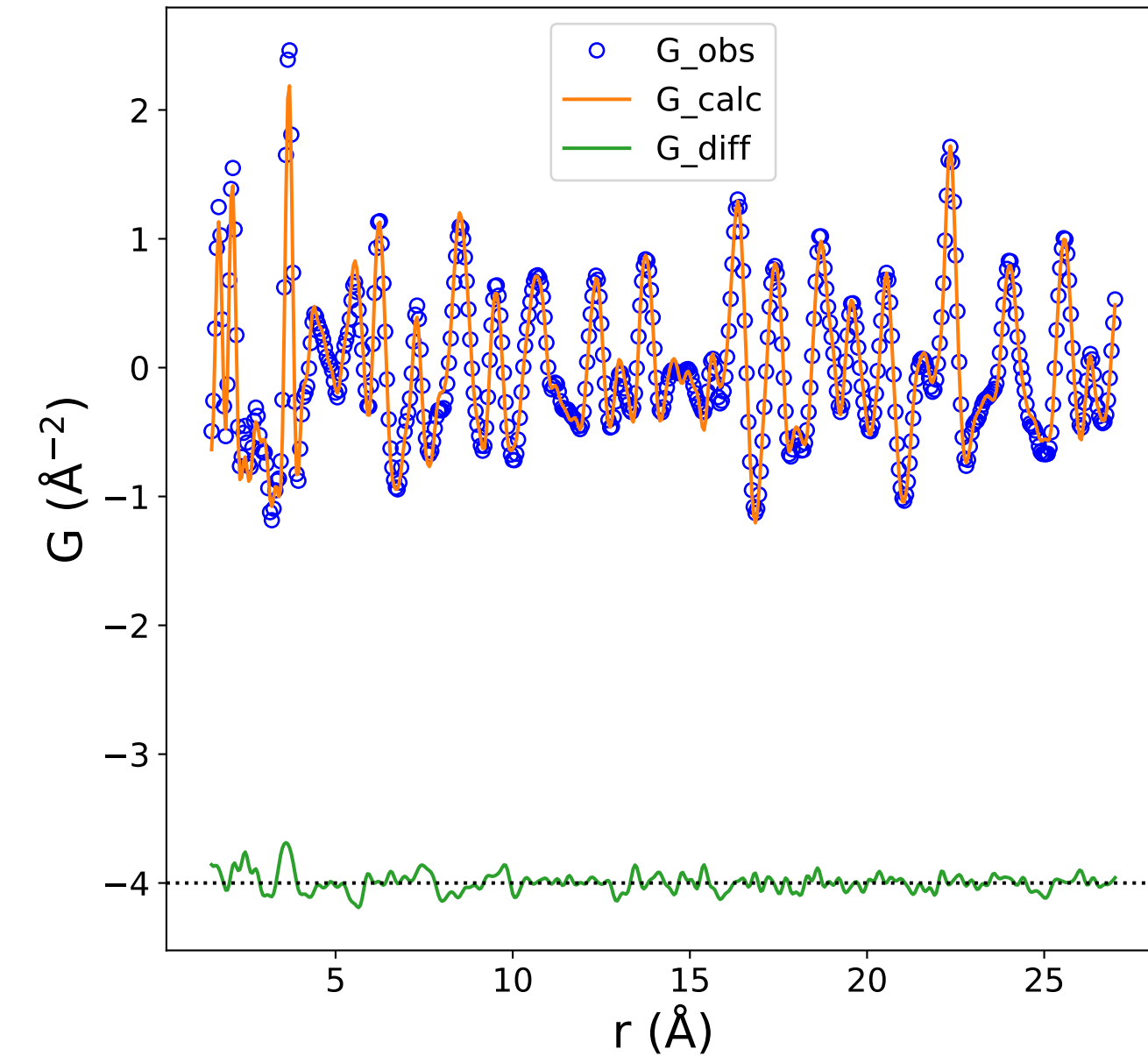
PDF Data and Fit (Rw = 0.127)
