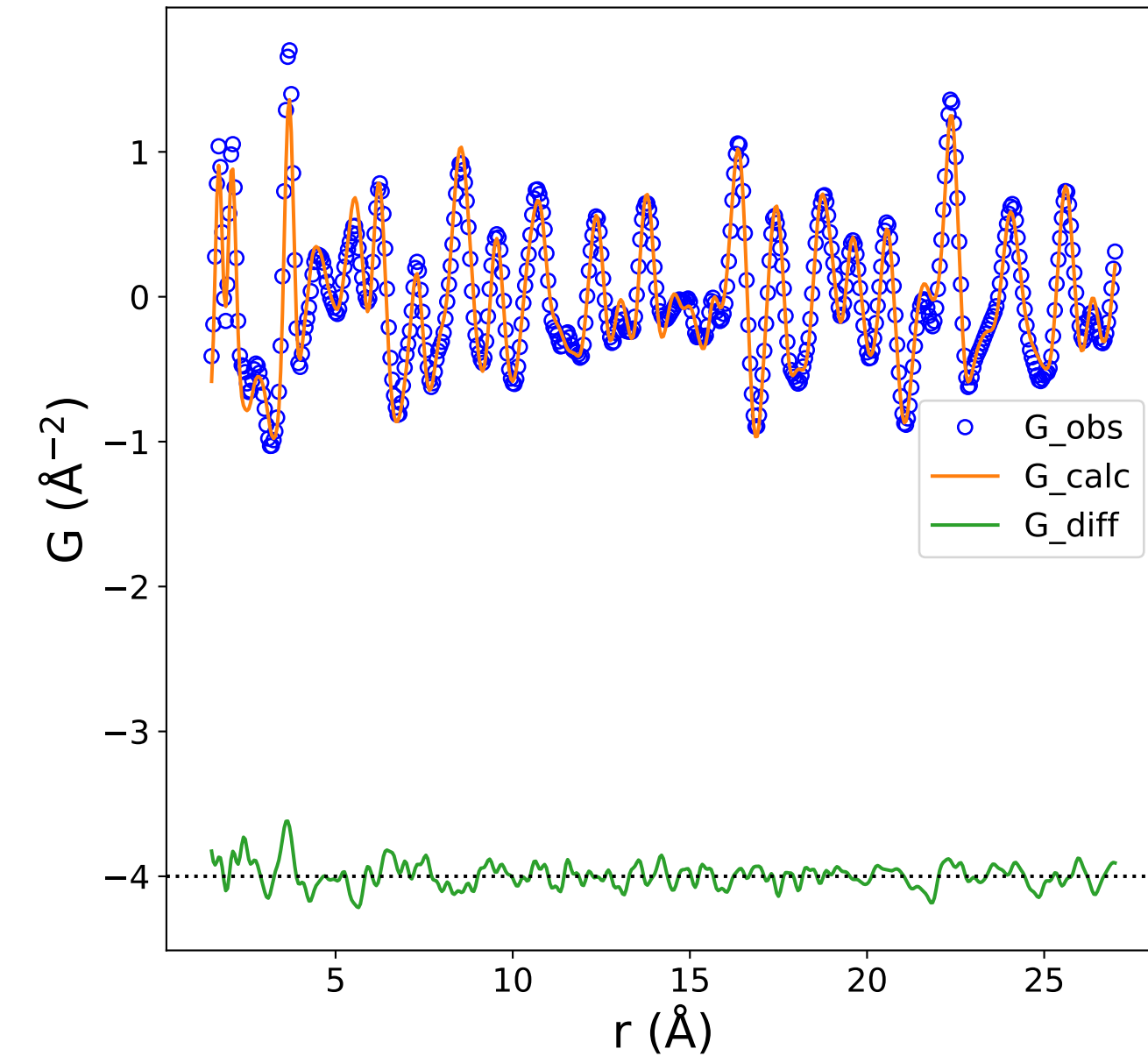
PDF Data and Fit (Rw = 0.183)
