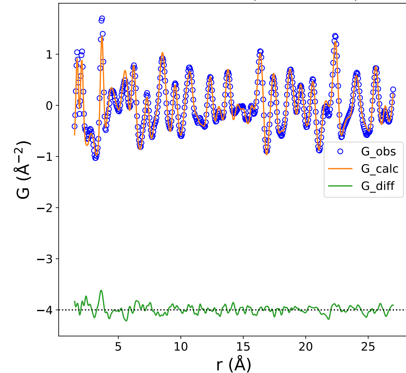
PDF Data and Fit (Rw = 0.182)
