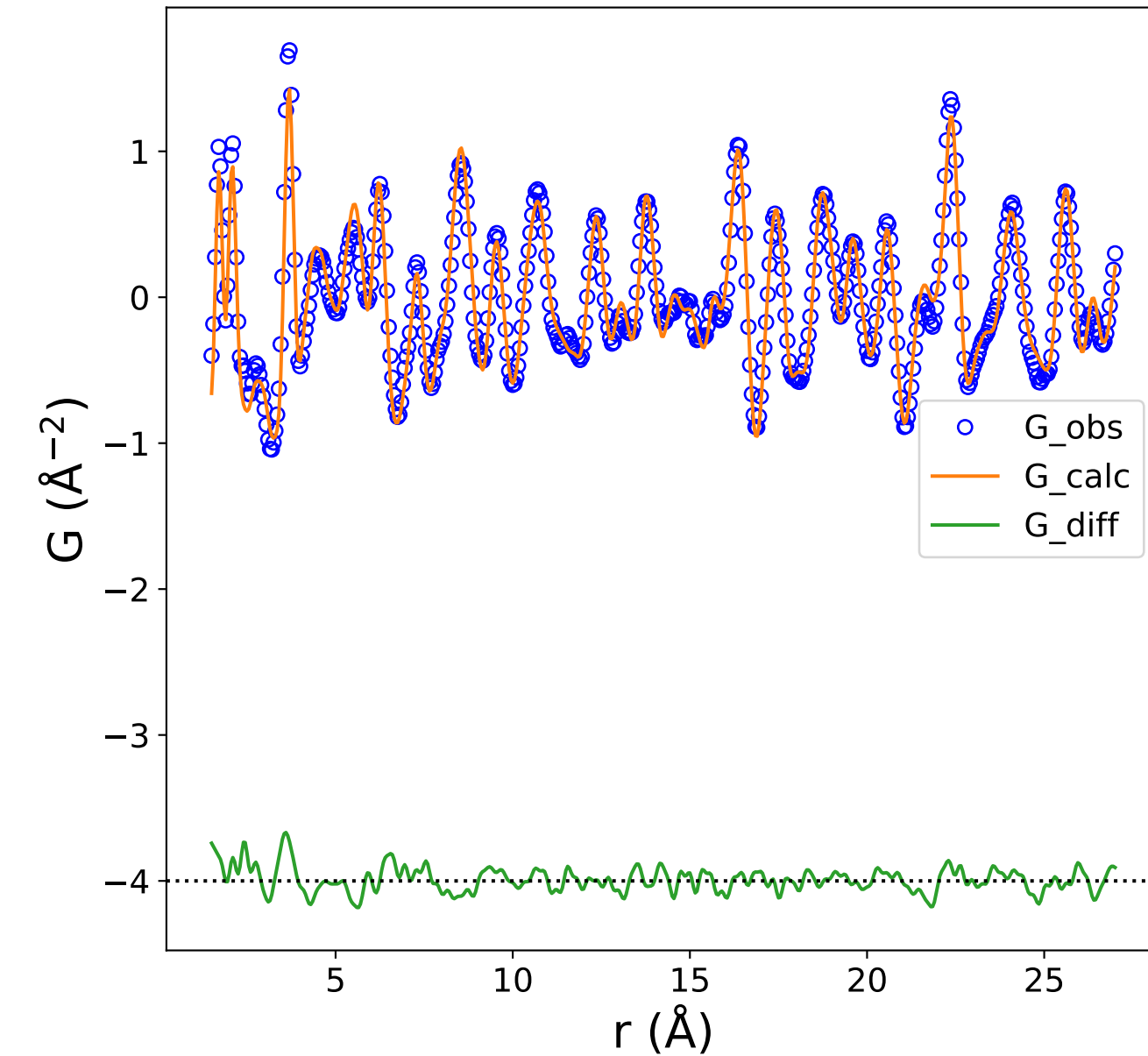
PDF Data and Fit (Rw = 0.181)
