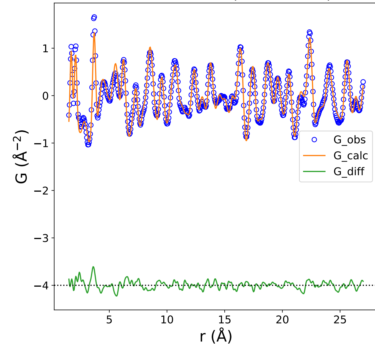
PDF Data and Fit (Rw = 0.188)
