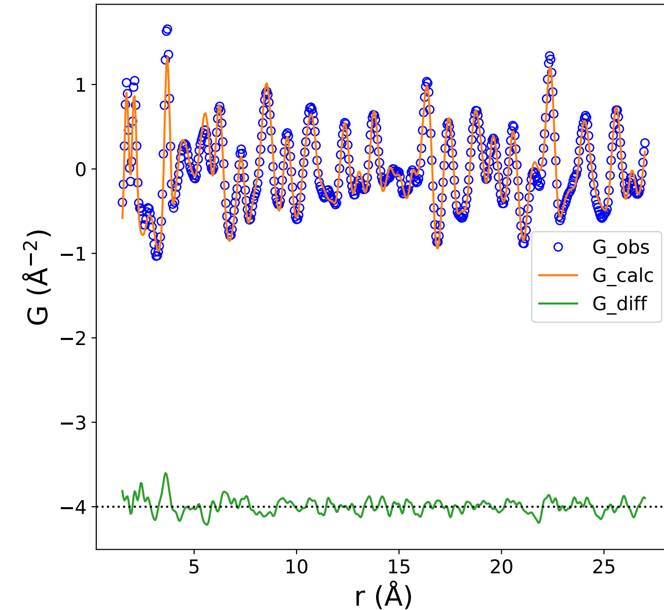
PDF Data and Fit (Rw = 0.189)
