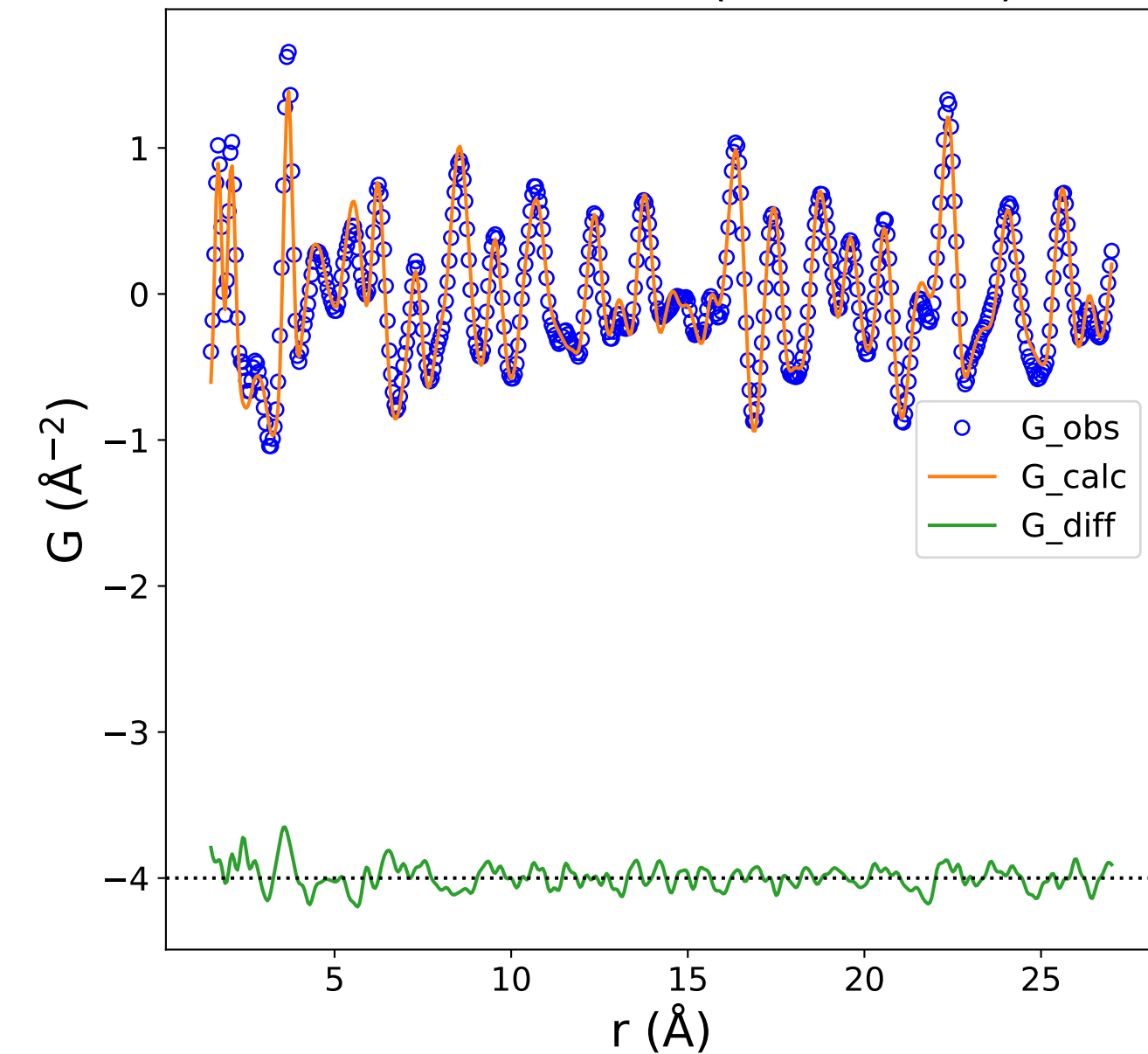
PDF Data and Fit (Rw = 0.184)
