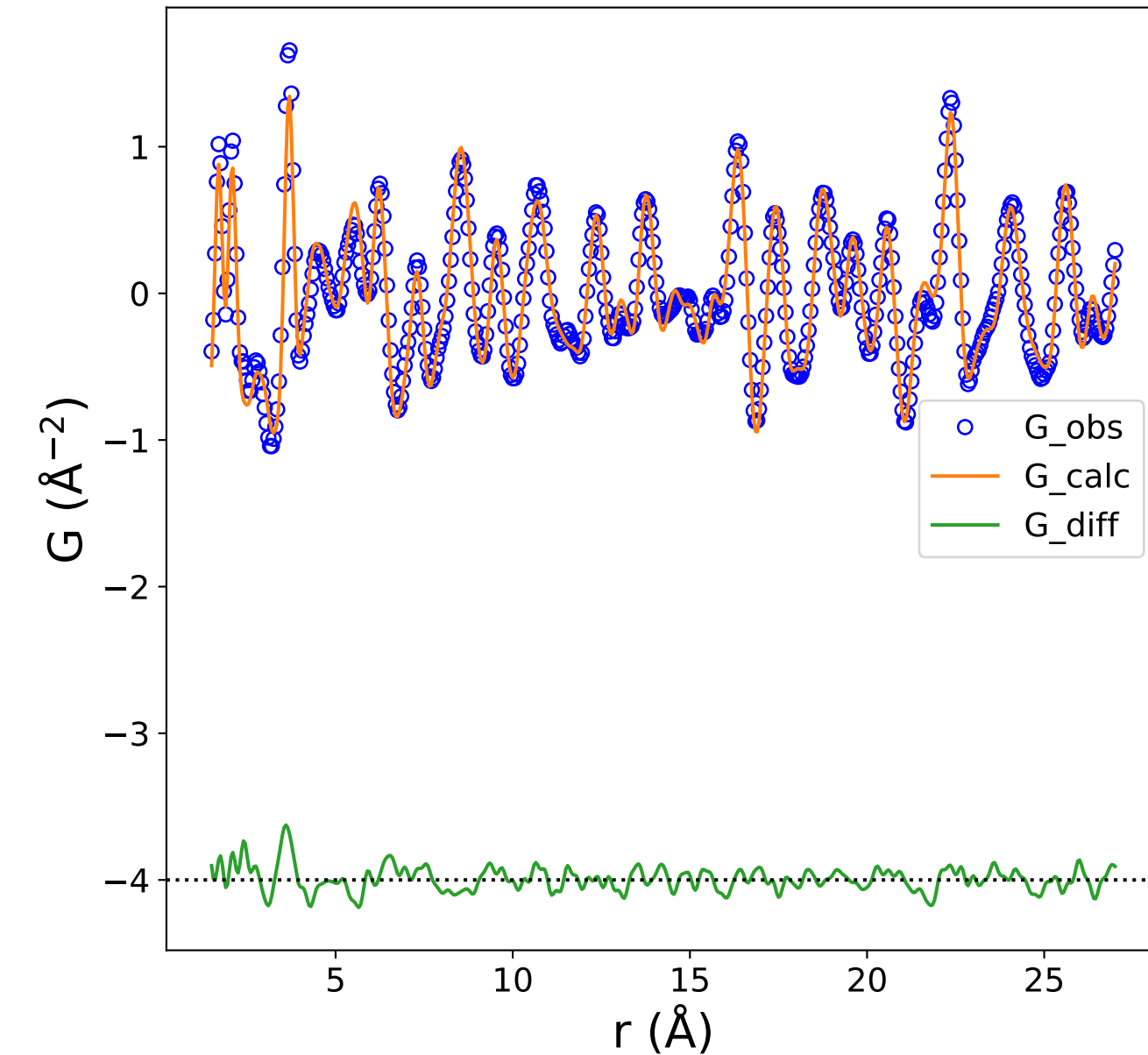
PDF Data and Fit (Rw = 0.180)
