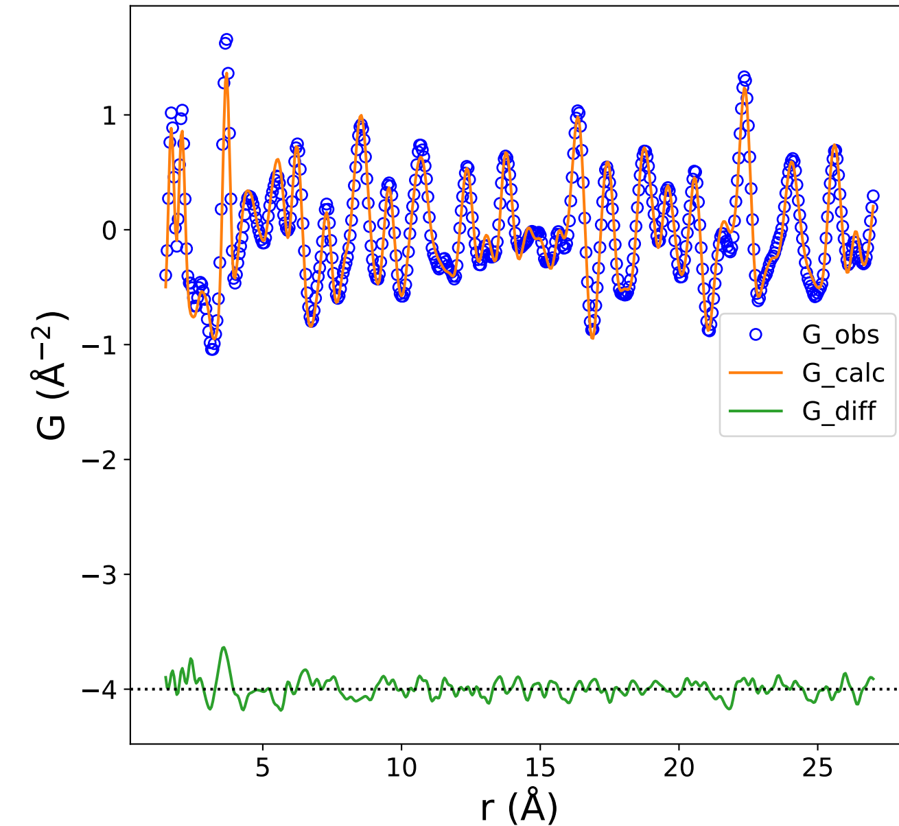
PDF Data and Fit (Rw = 0.179)
