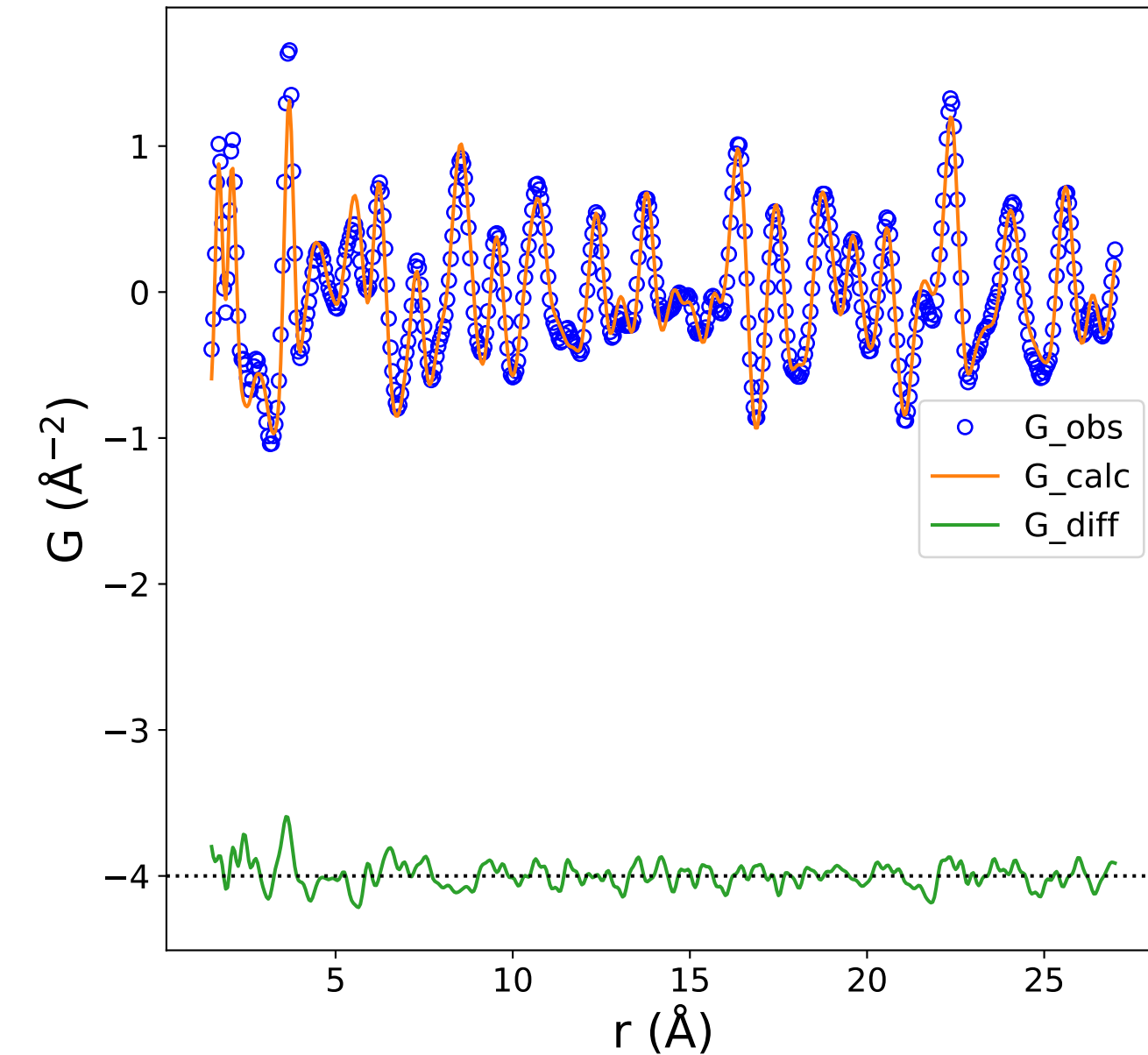
PDF Data and Fit (Rw = 0.193)
