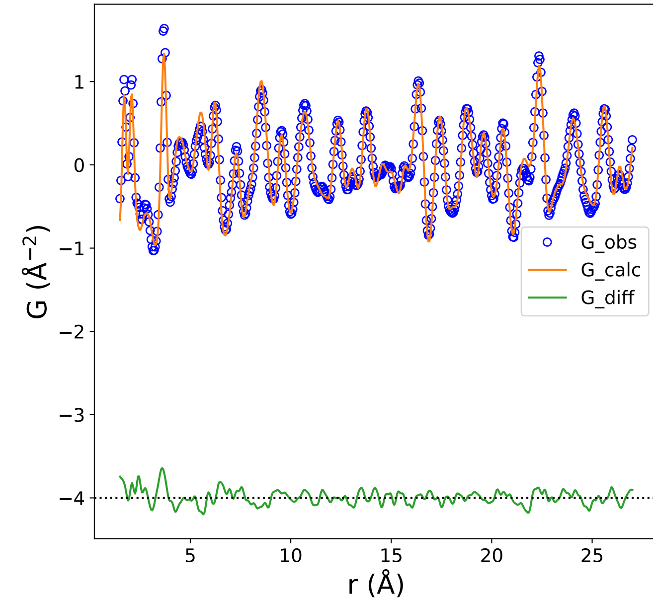
PDF Data and Fit (Rw = 0.192)
