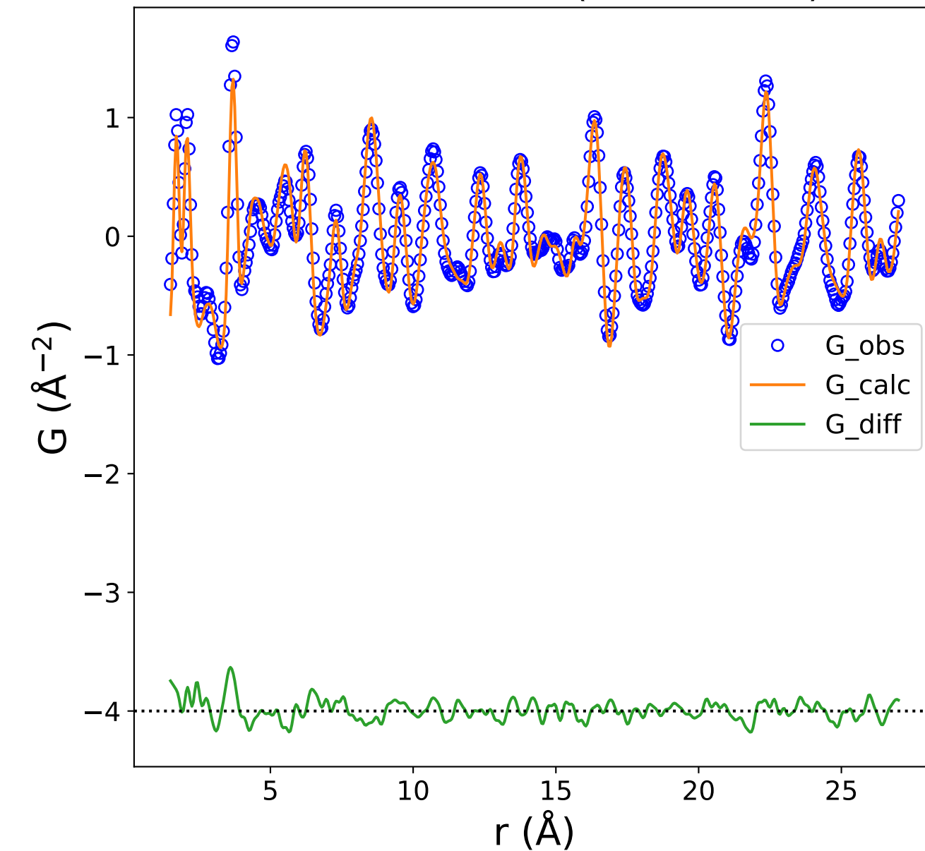
PDF Data and Fit (Rw = 0.187)
