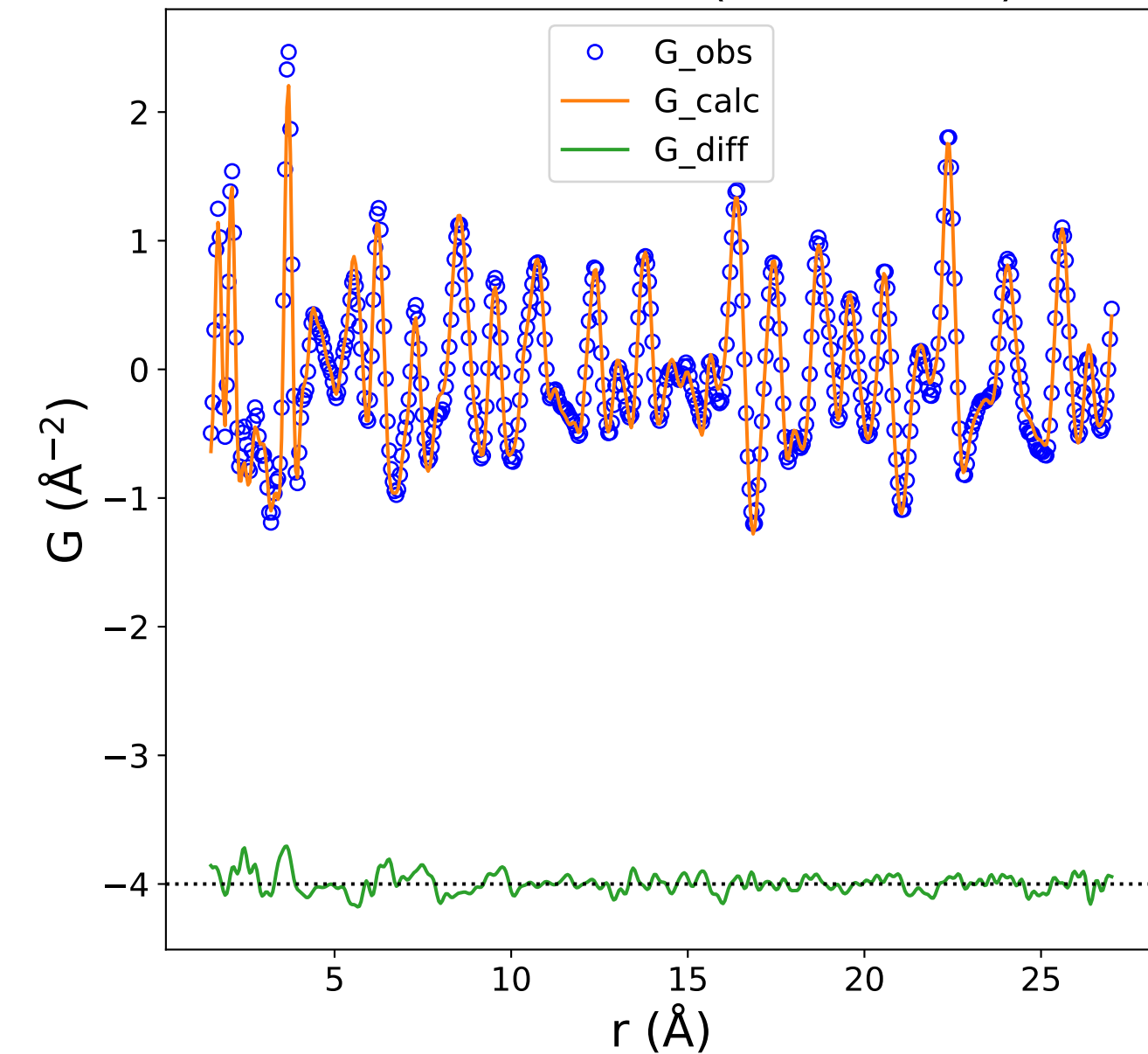
PDF Data and Fit (Rw = 0.129)
