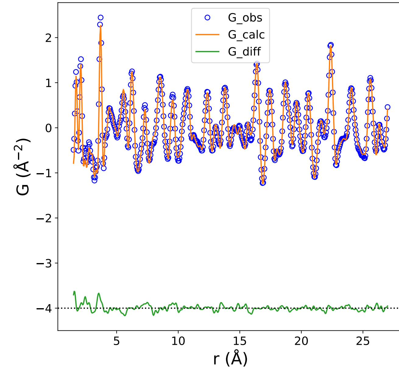
PDF Data and Fit (Rw = 0.121)
